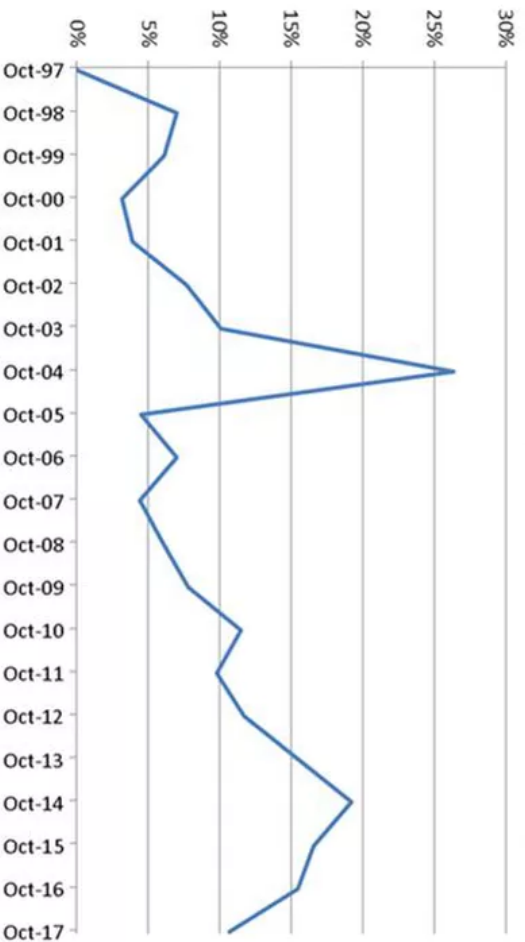
Figure 19: Pacific DC Intertie N-S TCC Outage May-October Yearly (1997-2017) 11
